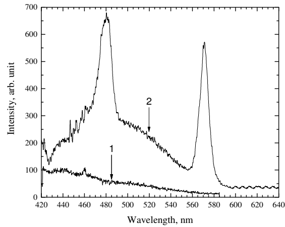
Fig. 4. The photoluminescence spectrum of opal sample infiltrated with dysprosium oxide: 1 – initial opal sample; 2 – opal sample infiltrated by dysprosium oxide.
